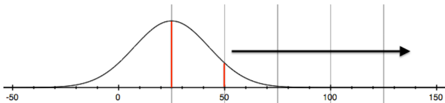
Figure 11 Illustration of a kernel density estimation calculation
