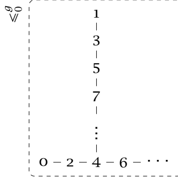
Figure 2 Induced pre-order for (5). The dashed box indicates R_0^f .
