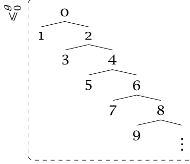
Figure 4 Induced pre-order for Example 1. The dashed box indicates R_0^f .
