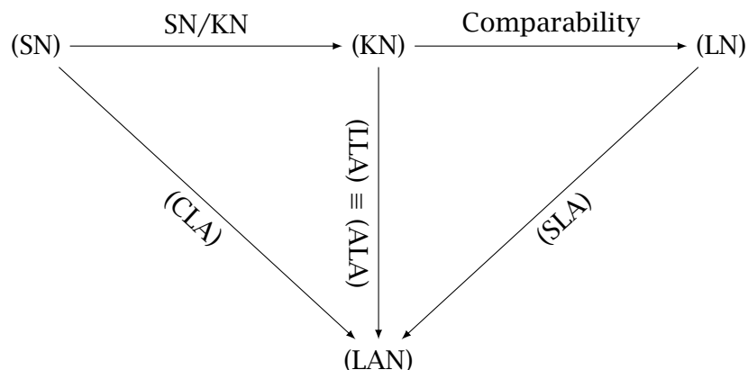
Figure 5 Four notions of necessity and the order properties that collapse them.
