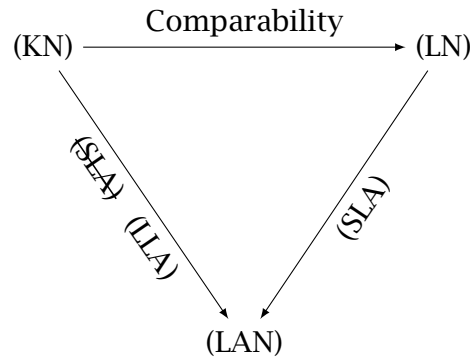
Figure 3 Three notions of necessity and the order properties that collapse them.
