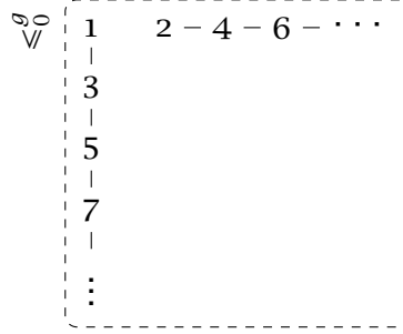
Figure 1 Induced pre-order for (3). The dashed box indicates R_0^f .
